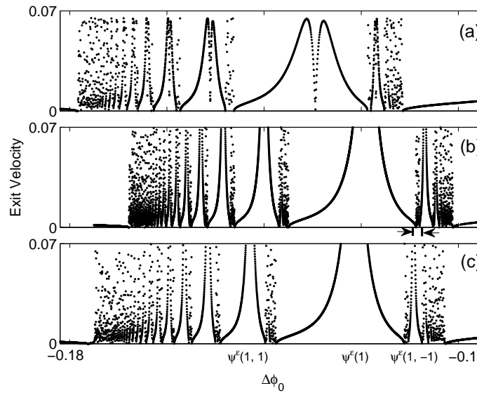
Figure 1: Comparisons of exit-velocity fractals from (a) PDE simulations, (b) ODE predictions, and (c) map predictions for the equal-amplitude initial conditions (16). ....
