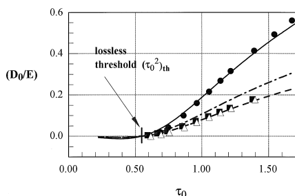
Fig. 1. Comparison of the ratio of the average dispersion to pulse energy, as given by Eq. (10b), with the results of numerical simulations of Eq. (3). Lossless case: solid – theory, circles – numerics. The threshold value (\tau_0^2)_{th} is marked with a tick mark. The following data pertain to the model with losses and amplification. L_{map} = L_{amp} , L_1/L_{amp} = 7/18 : dashed – theory, squares – numerics; L_{map} = L_{amp} , L_1/L_{amp} = 2/3 : triangles – numerics (see main text); L_{map} = L_1 + 4L_{amp} , L_1/L_{amp} = 0.5 : dash-dotted – theory (see main text).
