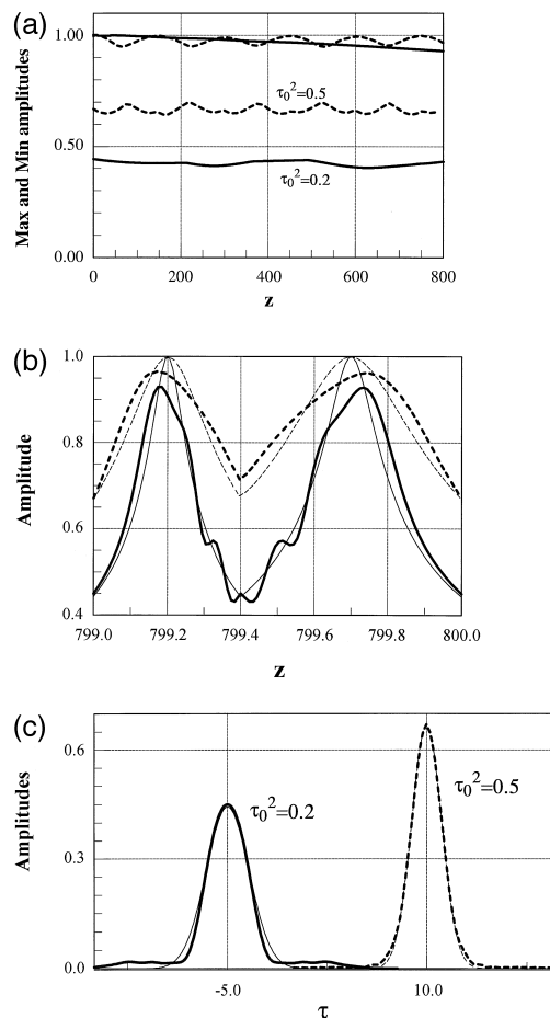
Fig. 2. (a) Evolution of minimum and maximum pulse amplitudes in the lossless case. Solid – \tau_0^2 = 0.2 ; dashed – \tau_0^2 = 0.5 . Other parameters are specified in the text. (b) Evolution of the pulse amplitude within one map period in the lossless case; 799 \leq z \leq 800 . Thick solid – \tau_0^2 = 0.2 ; thick dashed \tau_0^2 = 0.5 ; thin solid and thin dashed – the corresponding quantities for 0 \leq z \leq 1 . (c) Pulse profiles for the same parameters as in Fig. 2b. Thick solid – \tau_0^2 = 0.2 at z = 800 ; thick dashed – \tau_0^2 = 0.5 at z = 800 ; thin solid and thin dashed – the corresponding profiles at z = 0 . Note that in order to fit both profiles in the same figure, we shifted the centre of the pulse with \tau_0^2 = 0.2 from \tau = 0 to \tau = -5 , and the centre of the pulse with \tau_0^2 = 0.5 from \tau = 0 to \tau = 10 .
