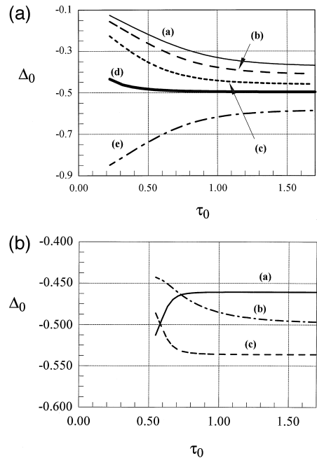
Fig. 3. (a) \Delta_0(\tau_0) for the case with L_{map} = L_{amp} for the following values of L_1/L_{amp} : 5/6 (a); 2/3 (b); 1/2 (c); 7/18 (d); 1/6 (e). (b) \Delta_0(\tau_0) for cases (i) and (ii). (a) – case (i) with any L_2/L_{amp} ; (b) – case (ii) with L_1/L_{amp} = 0.5 ; (c) – case (ii) with L_1/L_{amp} = 0.1 . Note that the vertical scale is different from that in Fig. 3a.
