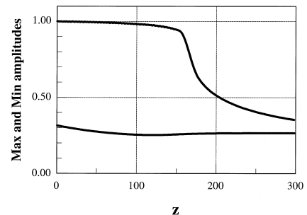
Fig. 4. Evolution of a pulse launched with \tau_0^2 = 0.1 and A = 1 in a line with D_0 = 0.305 (this value of D_0 corresponds to \tau_0^2 = 0.5 and A = 1 in Eq. (12b)). Note that the pulse energy is initially \sqrt{5} less than that of a pulse with \tau_0^2 = 0.5 and A = 1 , which would propagate stationarily at that average dispersion.
