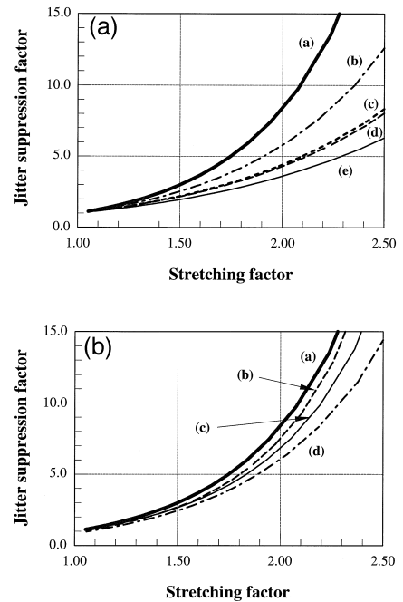
Fig. 5. (a) Jitter suppression factor calculated from Eq. (19). (a) – lossless case (also see main text). Other curves calculated for the case L_{\text{map}} = L_{\text{amp}} with the following values of L_1/L_{\text{amp}} : 1/2 (b); 1/6 (c); 2/3 (d); 5/6 (e). (b) Jitter suppression factor calculated from Eq. (19) for cases (i) and (ii). (a) – lossless case (shown for comparison); (b) – case (ii) with L_1/L_{\text{amp}} = 0.3 ; (c) – case (i) with any L_2/L_{\text{amp}} and case (ii) with L_1/L_{\text{amp}} = 0.1 ; (d) – case (ii) with L_1/L_{\text{amp}} = 0.5 .
