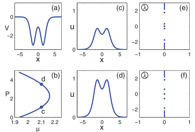
FIG. 1. (Color online) (a) Potential (31) in Example 1; (b) power curve of solitons; (c), (d) soliton profiles at points marked by the same letters in (b); (e), (f) stability spectra of solitons in (c) and (d).
