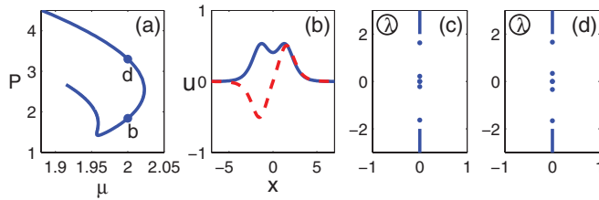
FIG. 2. (Color online) (a) Power curve of solitons in Example 2; (b) soliton profile at point “b” in (a) (solid and dashed lines for real and imaginary parts); (c),(d) stability spectra of solitons at points “b” and “d” in (a).
