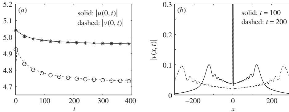
Figure 3. Numerical simulation of evolution of the embedded soliton under energy-enhancing perturbation (5.3) with a_1 = a_2 = 0.1 . (a) Evolutions of |u(0, t)| and |v(0, t)| . (b) Profile of |v(x, t)| at two values of t . Theoretical predictions for |u(0, t)| and |v(0, t)| found from (5.2) are shown in (a) by stars and circles, respectively.
