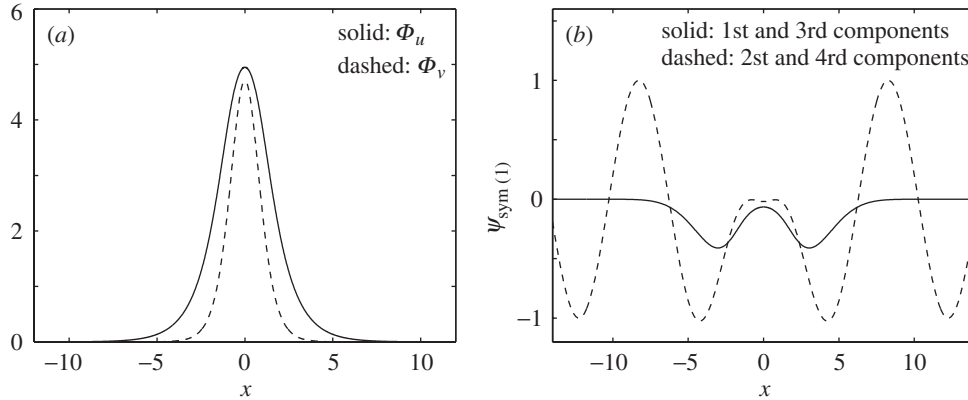
Figure 1. (a) The profile of an embedded soliton (\Phi_u(x), \Phi_v(x)) for the system (2.1), (2.2), with (2.14) and (5.1). The soliton exists at \omega_{\text{ES}} = 0.8114 . (b) The symmetric eigenfunction \psi_{\text{sym}(1)}(x) of the linearized problem (3.3) defined by the boundary condition (3.8).
