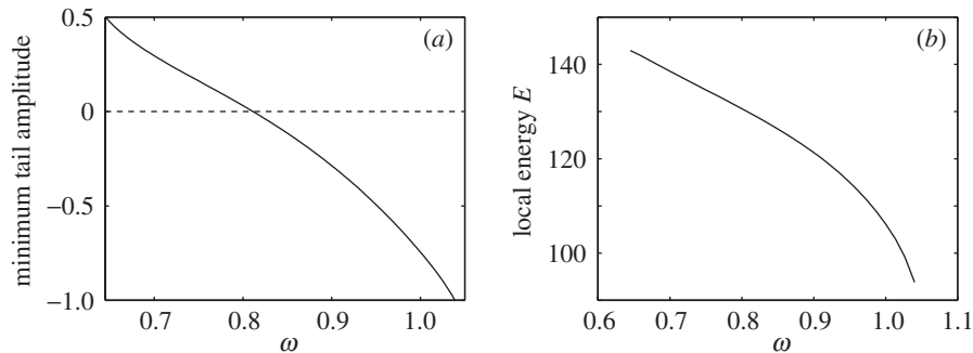
Figure 2. (a) The minimum tail amplitude r(\omega, \delta_{\text{min}}) of non-local waves (2.17) for various values of \omega in the system (2.1), (2.2), with (2.14) and (5.1). The phase \delta = \delta_{\text{min}} in (2.17) is chosen such that the amplitude r(\omega, \delta_{\text{min}}) is minimal. (b) Local energy curve E(\omega, \delta_{\text{rad}}) , as defined by (2.37).
