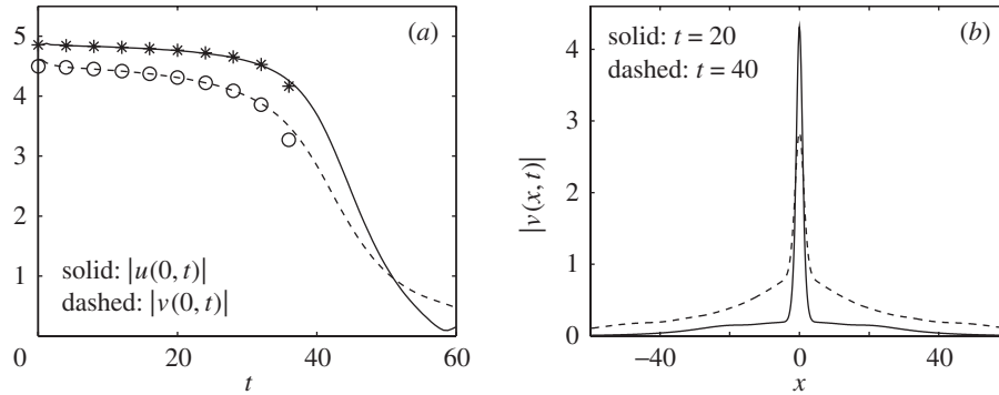
Figure 4. Numerical simulation of evolution of the embedded soliton under energy-reducing perturbation (5.3) with a_1 = a_2 = -0.1 . Shown are (a) evolutions of |u(0, t)| and |v(0, t)| and (b) profile of |v(x, t)| at two values of t . The theoretical prediction found from (5.2) are shown in (a) by stars and circles.
