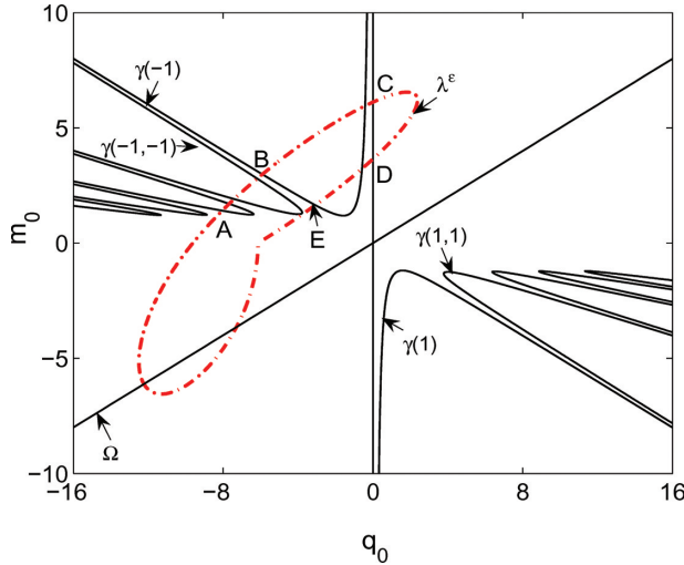
Figure 11. Singular curves of the map (13)–(14) for negative \varepsilon , as well as the initial-value curve \lambda^\varepsilon for unequal-amplitude initial conditions (21) with \varepsilon = -0.001 . Five of the intersections of \lambda^\varepsilon with singular curves are marked by letters ‘A, B, C, D, E’.
