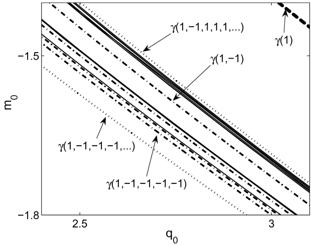
Figure 5. Amplification of the box region in Figure 4. The dash-dotted lines are \gamma(1, -1) , \gamma(1, -1, -1) , \gamma(1, -1, -1, -1) and \gamma(1, -1, -1, -1, -1) respectively from right to left. Accumulation curves \gamma(1, -1, -1, -1, \dots) and \gamma(1, -1, 1, 1, 1, \dots) are also shown.
