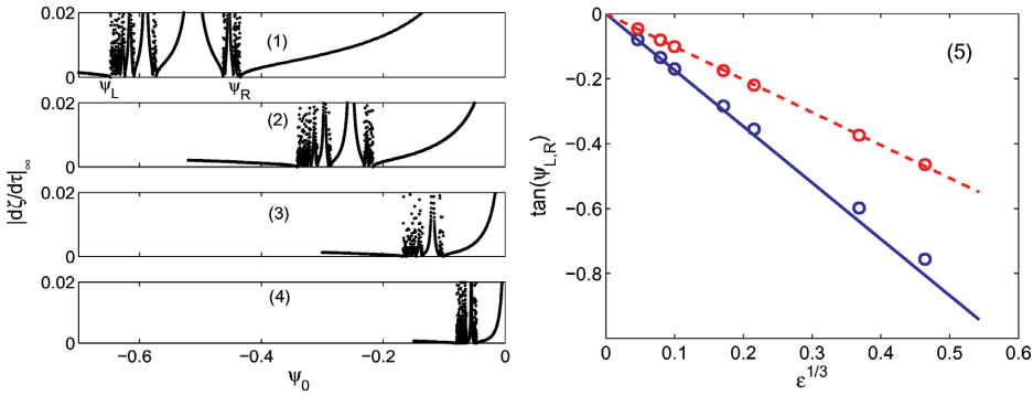
Figure 7. Left: Change of fractal structures in the ODEs (3) as \varepsilon \rightarrow 0^+ under the equal-amplitude initial condition (19). The \varepsilon values are (1) 0.1; (2) 0.01; (3) 0.001 and (4) 0.0001, respectively. Labels \psi_L and \psi_R represent the left and right boundaries of the fractal region. Right: \tan(\psi_L) (blue) and \tan(\psi_R) (red) versus \varepsilon^{1/3} . The circles are data from the ODE simulations, and the straight lines are the analytical formulae (46) from the map.
