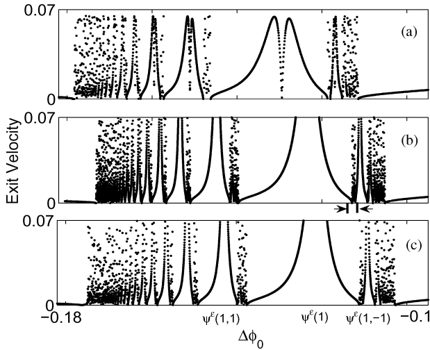
Figure 1. Comparisons of exit-velocity fractals from (a) PDE simulations, (b) ODE predictions, and (c) map predictions for the equal-amplitude initial conditions (16). The marked segment in (b) is amplified in Figure 10, where the solution dynamics in this segment is also shown. Labels \psi^\varepsilon(1) , \psi^\varepsilon(1, 1) , ... are locations of singularity peaks (of infinite height) in (c), which correspond to intersections of the initial-value curve \lambda^\varepsilon with the map's singular curves \gamma(1) , \gamma(1, 1) , ... in Figure 6 (see Section 4.1 for details).
