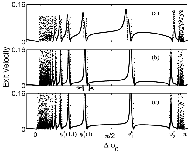
Figure 2. Comparisons of exit-velocity fractals from (a) PDE simulations, (b) ODE predictions, and (c) map predictions for the unequal-amplitude initial conditions (17). For the segment of structures marked in (b), its movement with varying values of \varepsilon is displayed in Figure 9. Labels \psi_1^\varepsilon , \psi_1^\varepsilon(1) , ... are locations of singularity peaks in (c) which correspond to intersections of the initial-value curve \lambda^\varepsilon with the map's singular curves \gamma_0 , \gamma(1) , ... in Figure 8 (see Section 4.2 for details).
