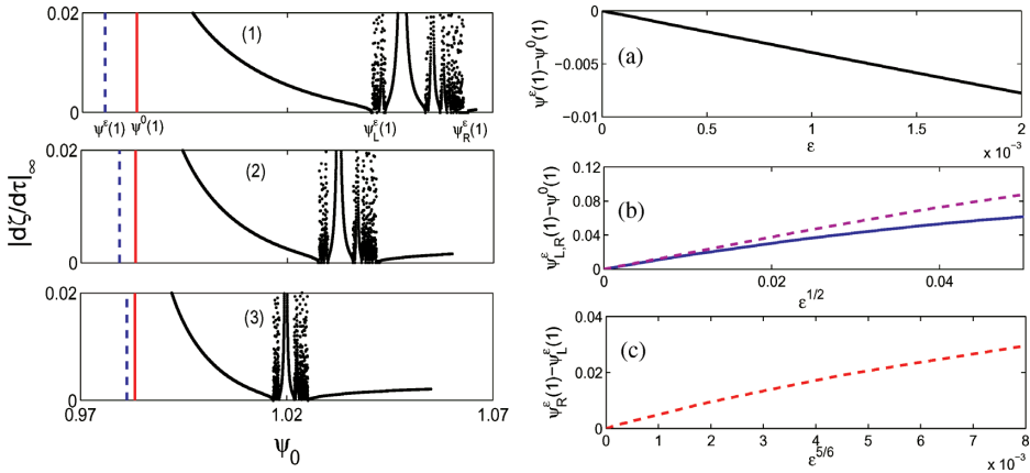
Figure 9. Left: Segments of the ODEs fractal structures near the lower intersection between \lambda^\varepsilon and the primary singular curve \gamma(1) under unequal-amplitude initial conditions (21) [this segment for \varepsilon = 0.001 was marked in the whole fractal structure of Figure 2(b)]. The \varepsilon values are (1) 0.002; (2) 0.001 and (3) 0.0005. Right: (a) \psi^\varepsilon(1) - \psi^0(1) versus \varepsilon ; (b) \psi_L^\varepsilon(1) - \psi^0(1) (blue) and \psi_R^\varepsilon(1) - \psi^0(1) (red) versus \varepsilon^{1/2} ; (c) \psi_R^\varepsilon(1) - \psi_L^\varepsilon(1) versus \varepsilon^{5/6} .
