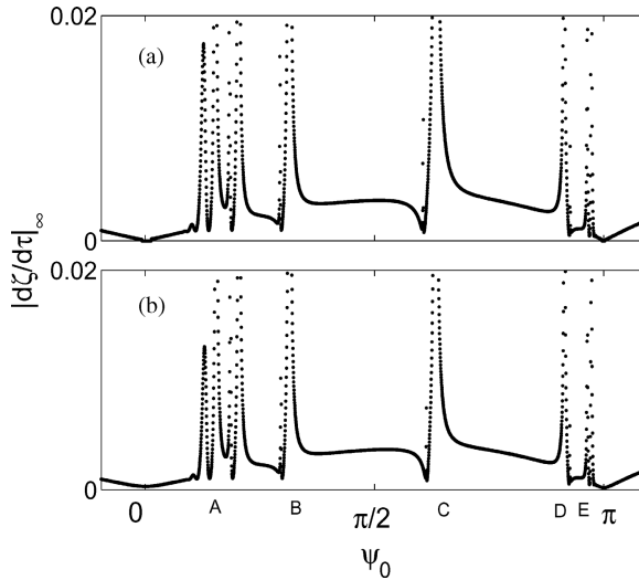
Figure 12. Comparison of the exit-velocity graphs from (a) ODE predictions, and (b) map predictions for \varepsilon = -0.001 . The initial conditions of the ODEs are (21) for unequal-amplitude initial waves. Letters “A, B, . . .” are locations of some singularity peaks in (b), which correspond to the intersections of \lambda^\varepsilon with singular curves in Figure 11 (marked by the same letters).
