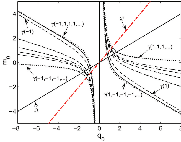
Figure 6. Curve \lambda^\epsilon of the map's initial points (45) which corresponds to the equal-amplitude initial conditions (16). Some singular curves are also shown. The dashed curves are the same as those in Figure 4, and the solid curves are \gamma(1, -1) and \gamma(-1, 1) .
