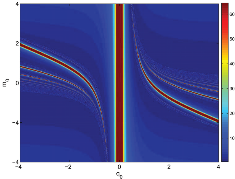
Figure 3. Values of |m_\infty| in the initial-value space (q_0, m_0) for the map (13)–(14) with \text{sgn}(\varepsilon) = 1 . Colors represent value levels of |m_\infty| .
