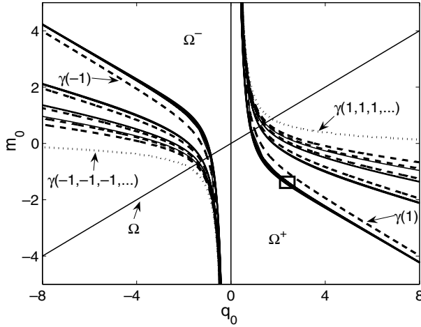
Figure 4. Plots of singular curves \gamma(a_0) , \gamma(a_0, a_1) , \gamma(a_0, a_1, a_2) , \gamma(a_0, a_1, a_2, a_3) , and \gamma(a_0, a_1, a_2, a_3, a_4) for all binary numbers of a_0, \dots, a_4 . The dashed lines in the right plane are \gamma(1) , \gamma(1, 1) , \gamma(1, 1, 1) , \gamma(1, 1, 1, 1) and \gamma(1, 1, 1, 1, 1) respectively from left to right. The accumulation curve \gamma(1, 1, 1, \dots) is also shown (as dotted lines). Lines in the left half plane are similar. The box region will be magnified in Figure 5.
