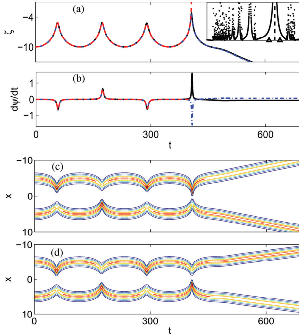
Figure 10. Dynamics of the ODE and PDE solutions on the hill of binary sequence \mathbf{a} = (1, -1, 1) in the exit-velocity fractals for equal-amplitude initial conditions (16). The inset in (a) is an amplification of the segment marked in the ODE fractal of Figure 1(b), where the widest hill is the one of binary sequence \mathbf{a} = (1, -1, 1) . Three locations \psi_a < \psi_b < \psi_c on this hill are marked by two triangles and a vertical dashed line, with the dashed line at \psi_b being the singularity peak point. The ODE solutions at \psi_a, \psi_b and \psi_c are plotted as dash-dotted lines (blue), dashed lines (red) and solid lines (black) in (a, b), respectively. The PDE solutions at points corresponding to \psi_a and \psi_c in the PDE fractal of Figure 1(a) are shown in (c, d), respectively (contour plots).
