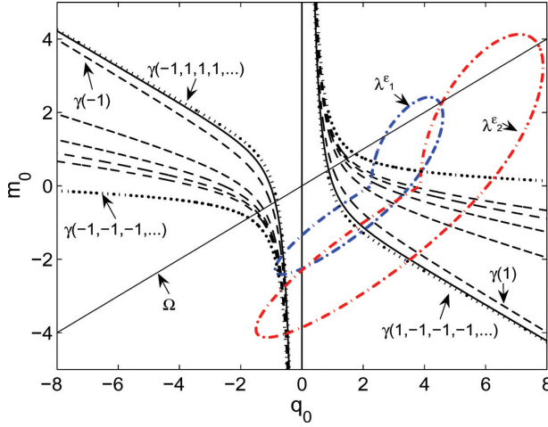
Figure 8. Curves of the map's initial points (47) corresponding to the unequal-amplitude initial conditions (21) at two \varepsilon values: \varepsilon_1 = 0.01 (blue) and \varepsilon_2 = 0.005 (red). Some singular curves are also shown by the same notations as in Figure 6.
