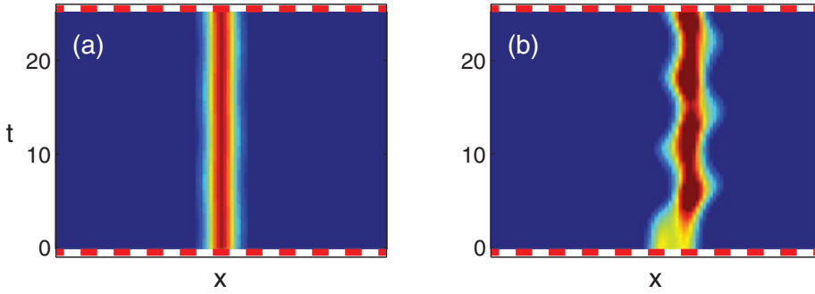
Figure 3. Nonlinear evolutions of the on-site (a) and off-site (b) solitary waves in Figure 1(b,d) under phase-gradient perturbations (89). Red bars represent locations of high nonlinear-lattice values.
