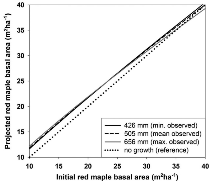
Fig. 5. The influence of mean growing season precipitation on projected red maple basal area based on eq. 2. All other variables in the model were held fixed at the sample mean ( dt = 6.2 , dq = 24.1 cm, pctrm = 0.81 , age = 77 years). dt, growth interval length; dq, plot quadratic mean diameter; pctrm, proportion of basal area comprised of red maple.
